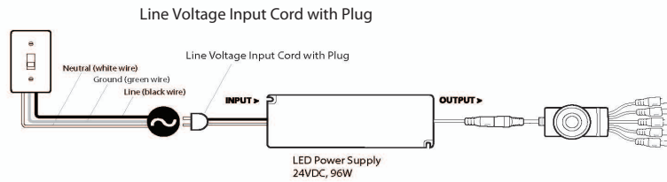
Typical Application
