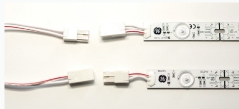
Power Lead Kit 100 mm
