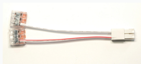
Connector Lead Kit
