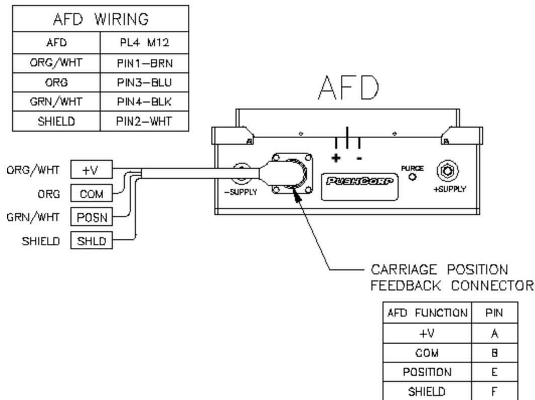
FIGURE 4: EXTERNAL I/O CONNECTIONS
