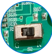
Integrated toggle switch for red and green LED
