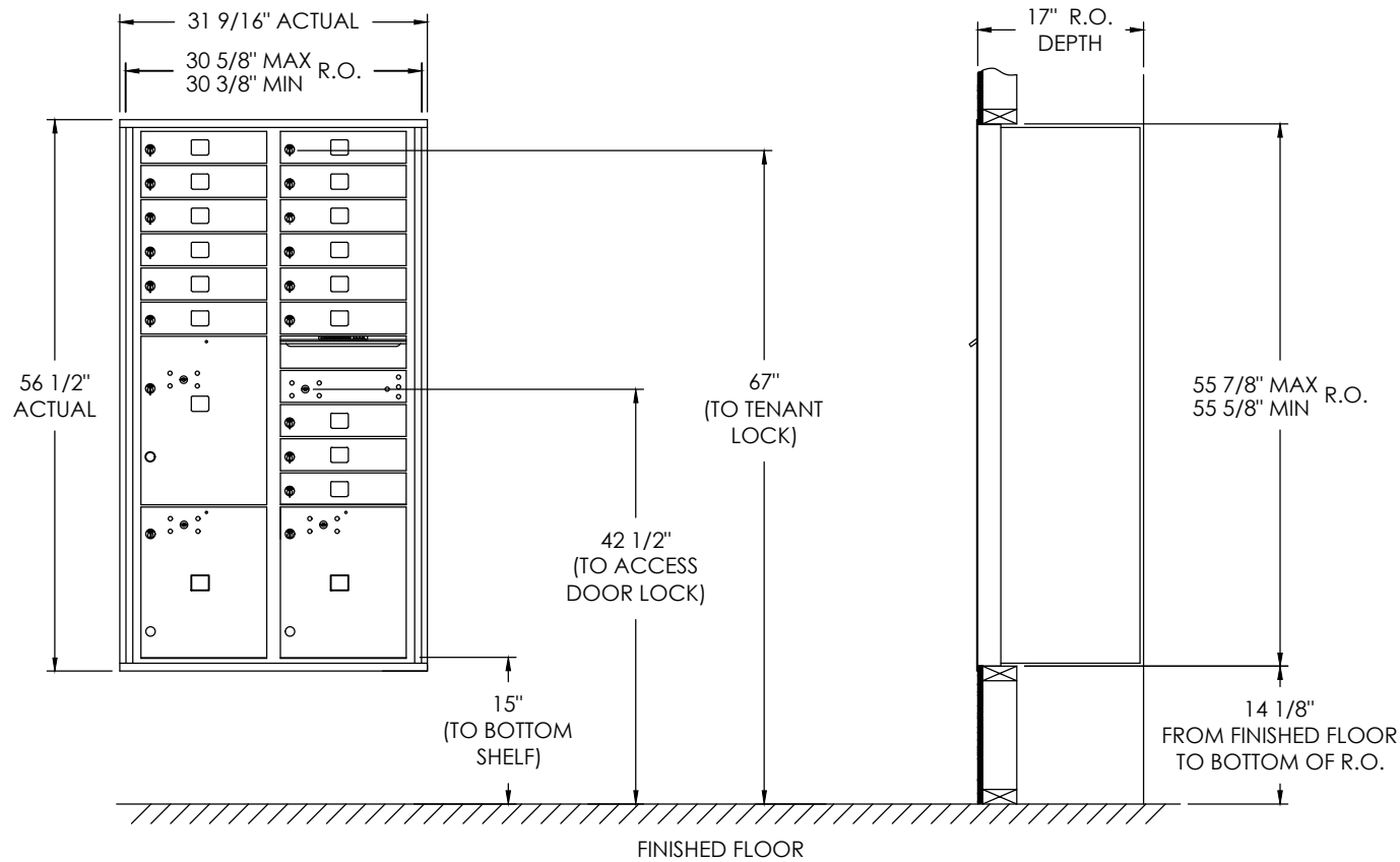
COMPARTMENT CHART
