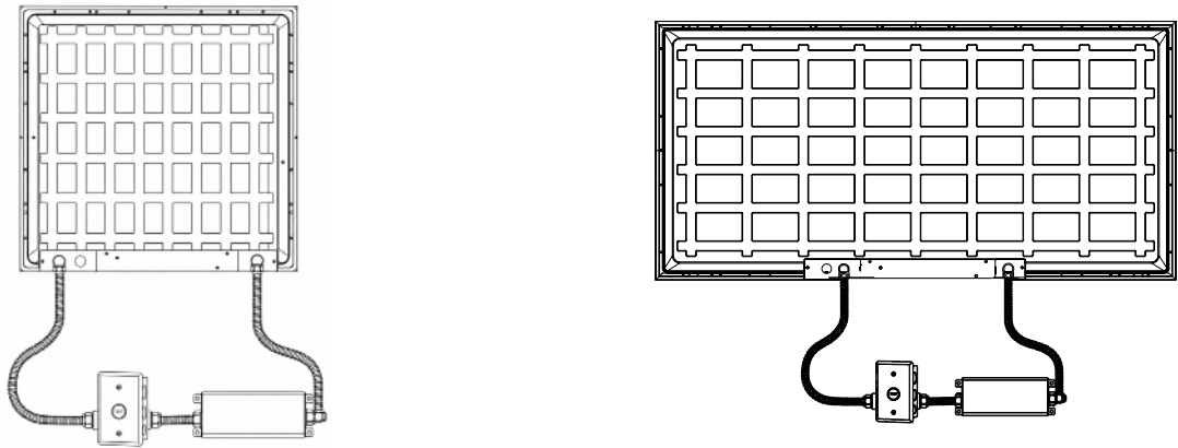
View of top with E3 (8W-Quick Ship) Emergency pack
