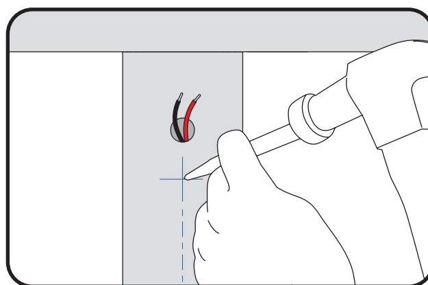
② Use center punch and hammer to create a dimple over the two marked locations.
