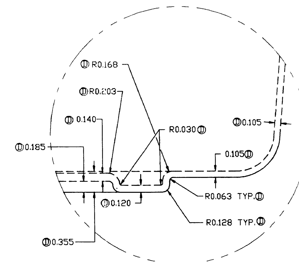
SECTION "B-B" FULL SCALE
