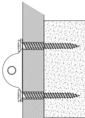
FIGURE A DRYWALL W/STUDS
