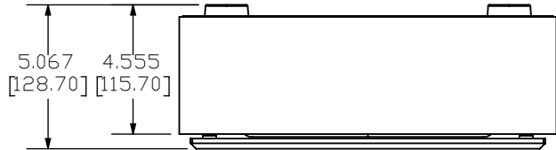
UP-FIRING VERSION
