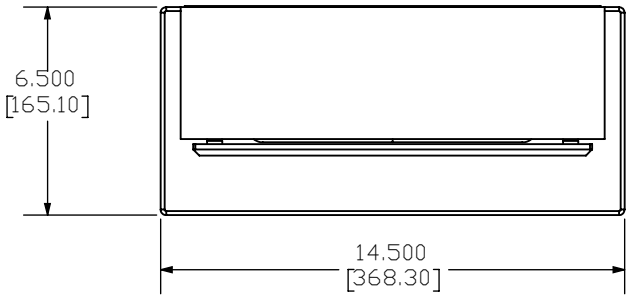
PEDESTAL VERSION
