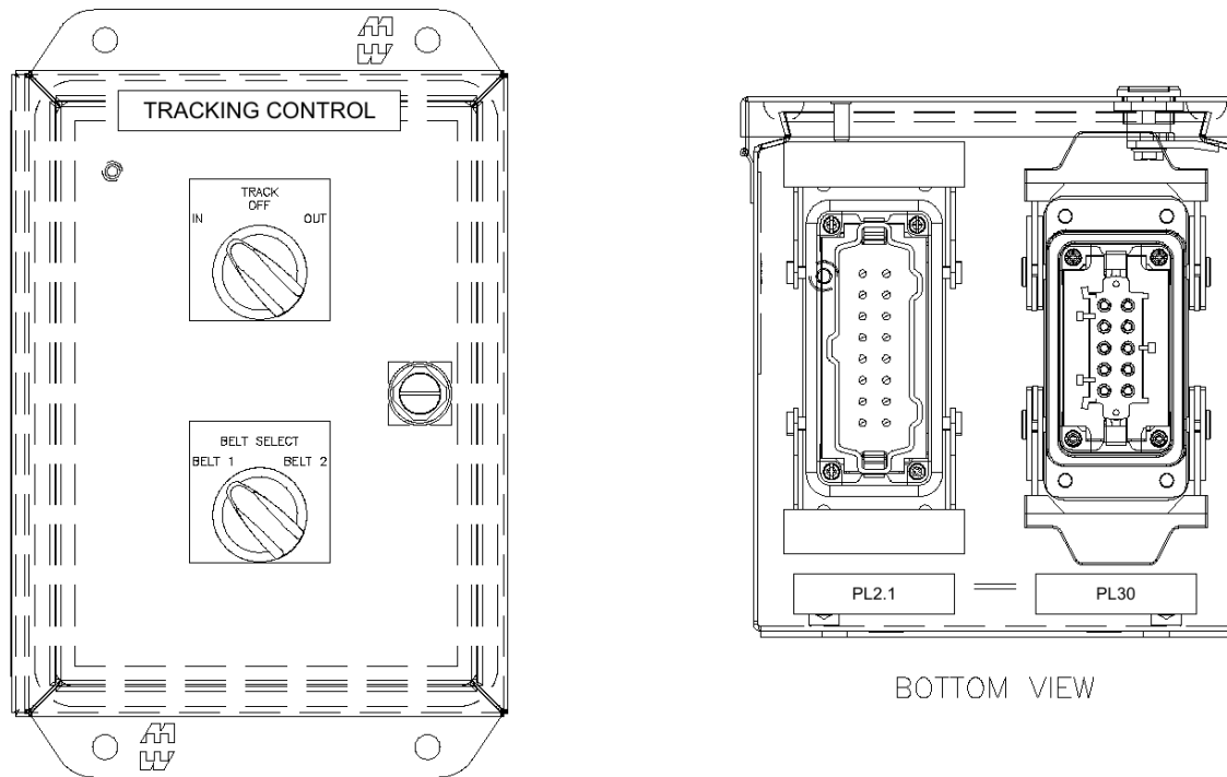
Figure 6: Tracking Control Box
