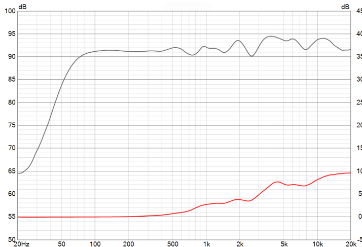
HORN SPL
