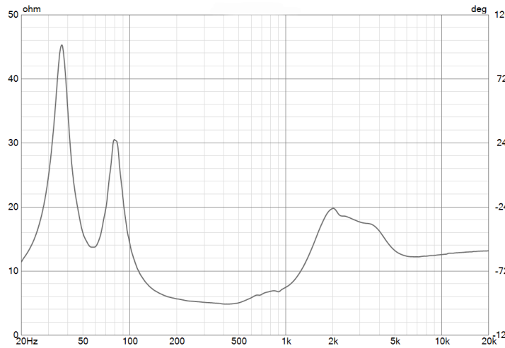
HORN IMPEDANCE
