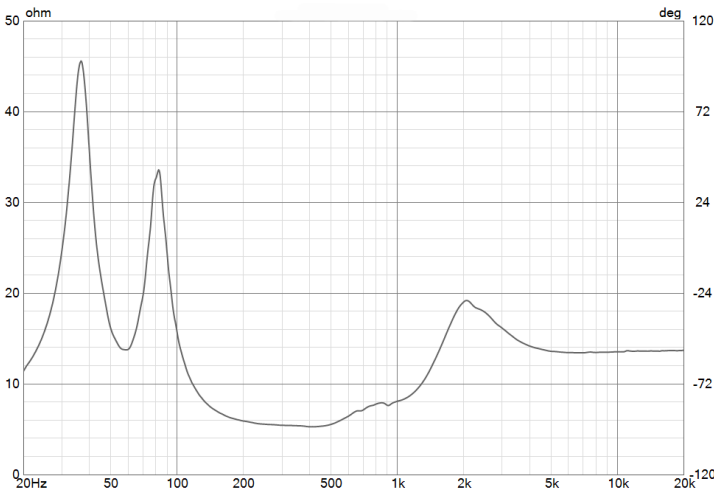
COLLAR IMPEDANCE
