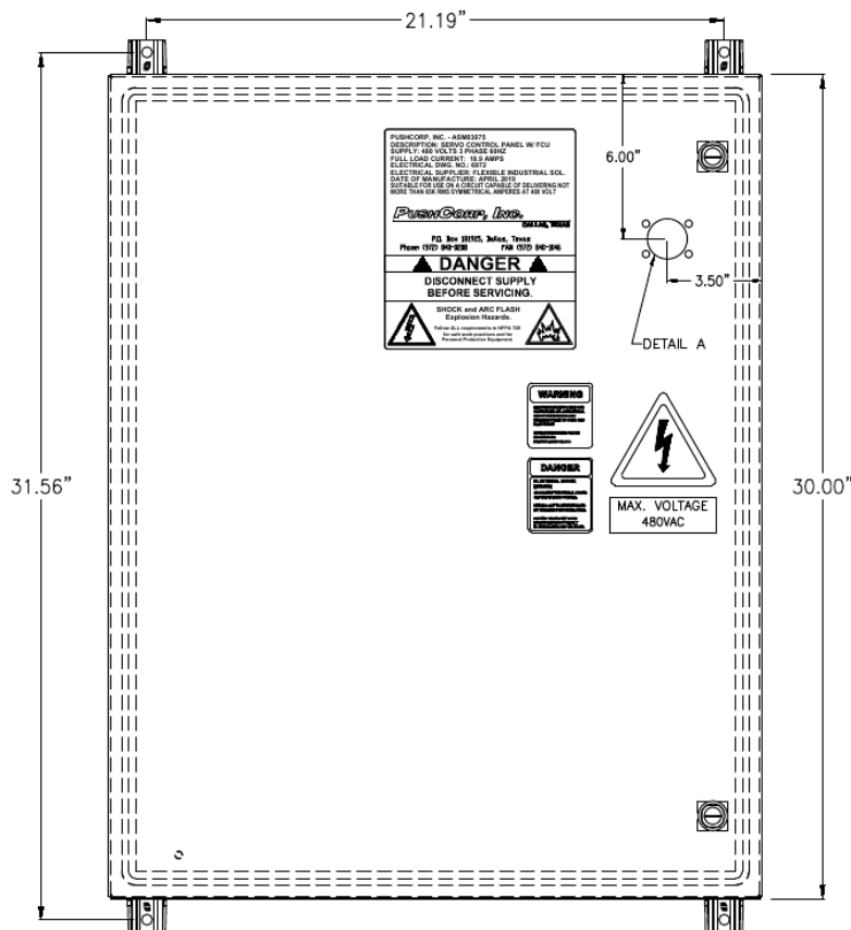
Figure 1. Cabinet Mounting
