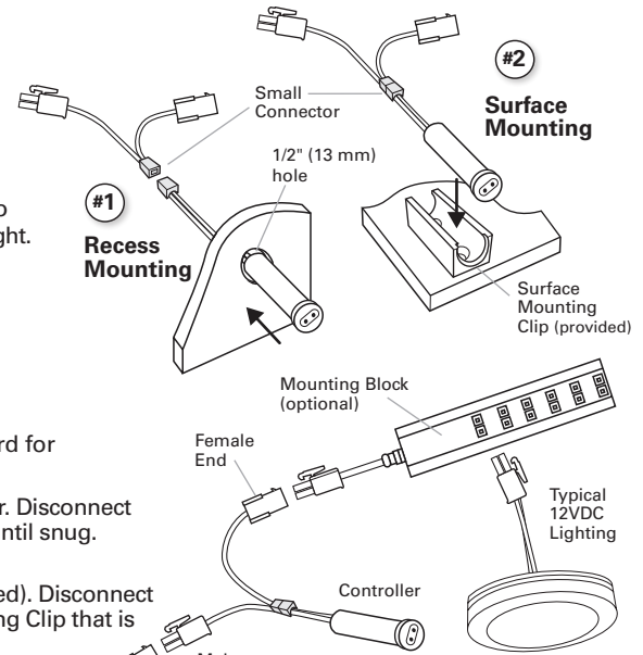
12VDC OPTION 1
