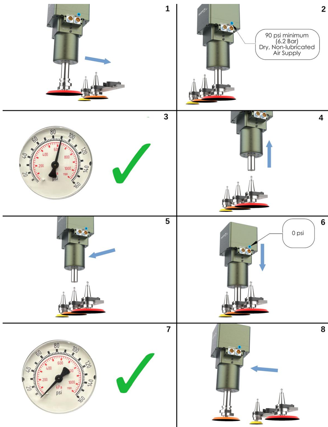
Figure 16: STC Spindle Tool Change Sequence
