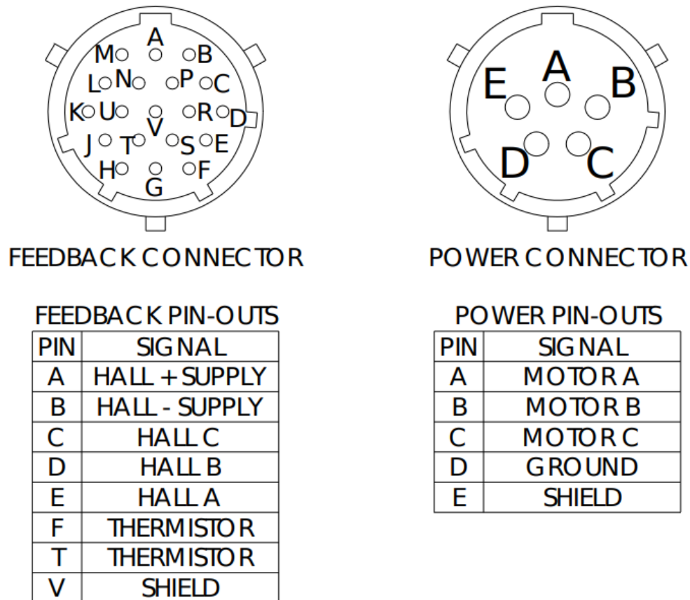
Figure 12: Electrical Connector Pin-Outs
