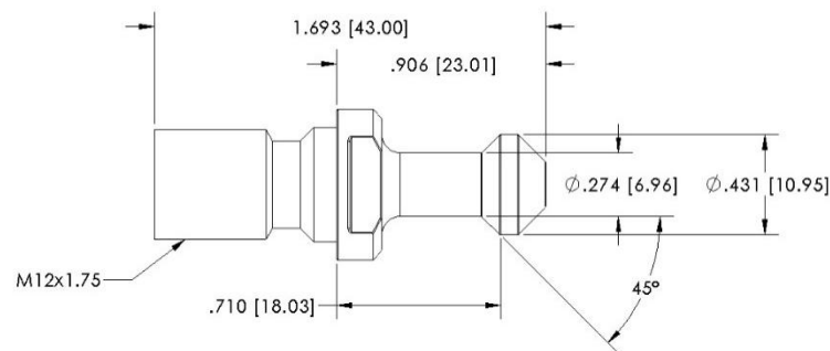
Figure 8: BT30 Retention Knob
