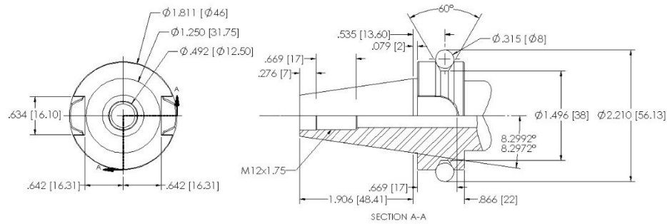
Figure 7: STC-BT30 Toolholder Dimensions
