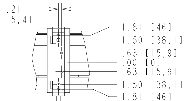
DETAIL A SCALE 0.300
