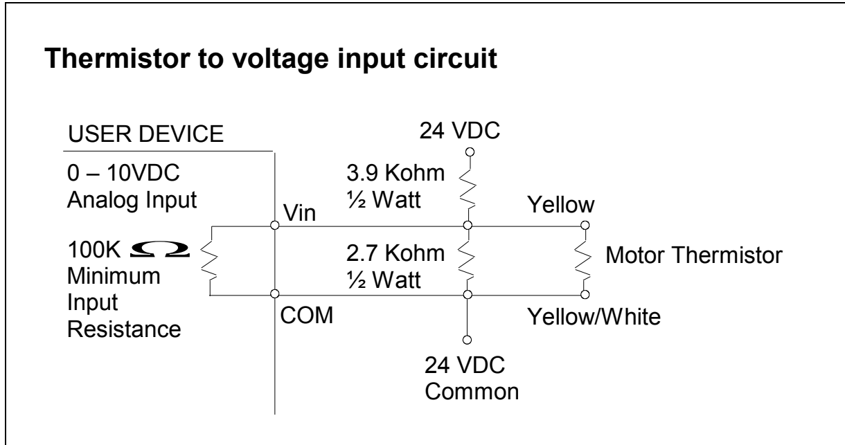
Figure 4. Thermistor Circuit
