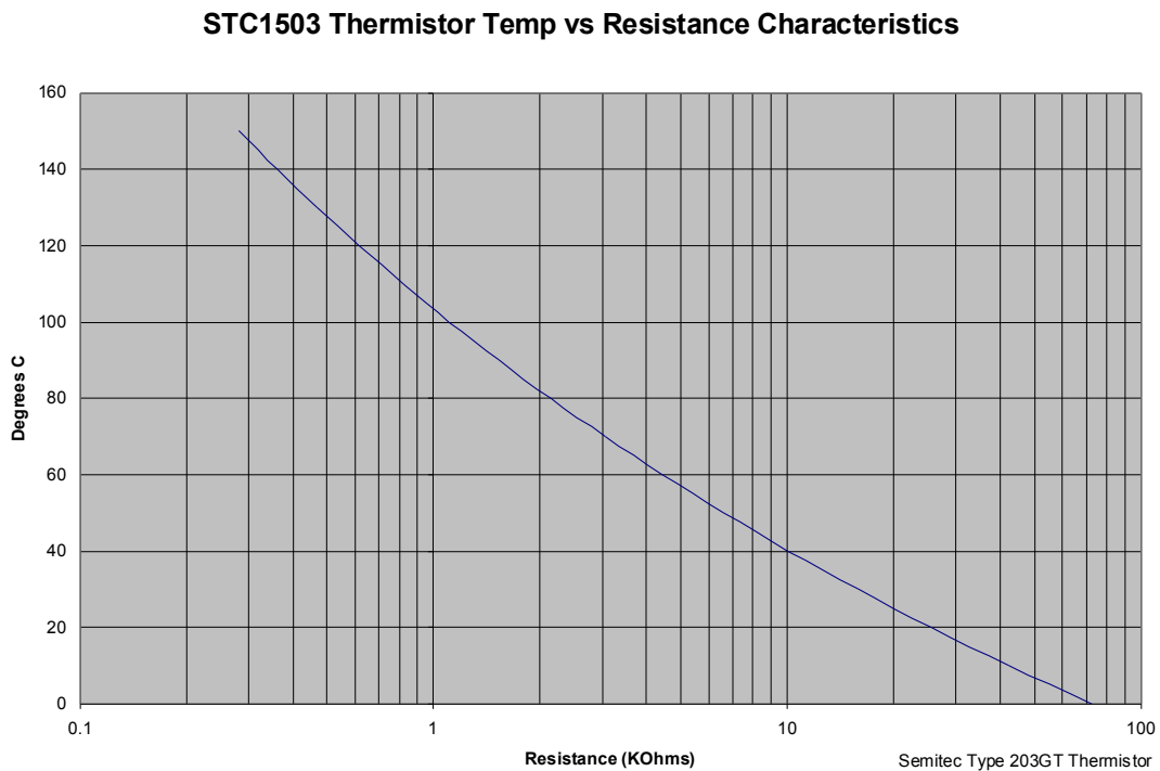
Figure 3. Thermistor Chart
