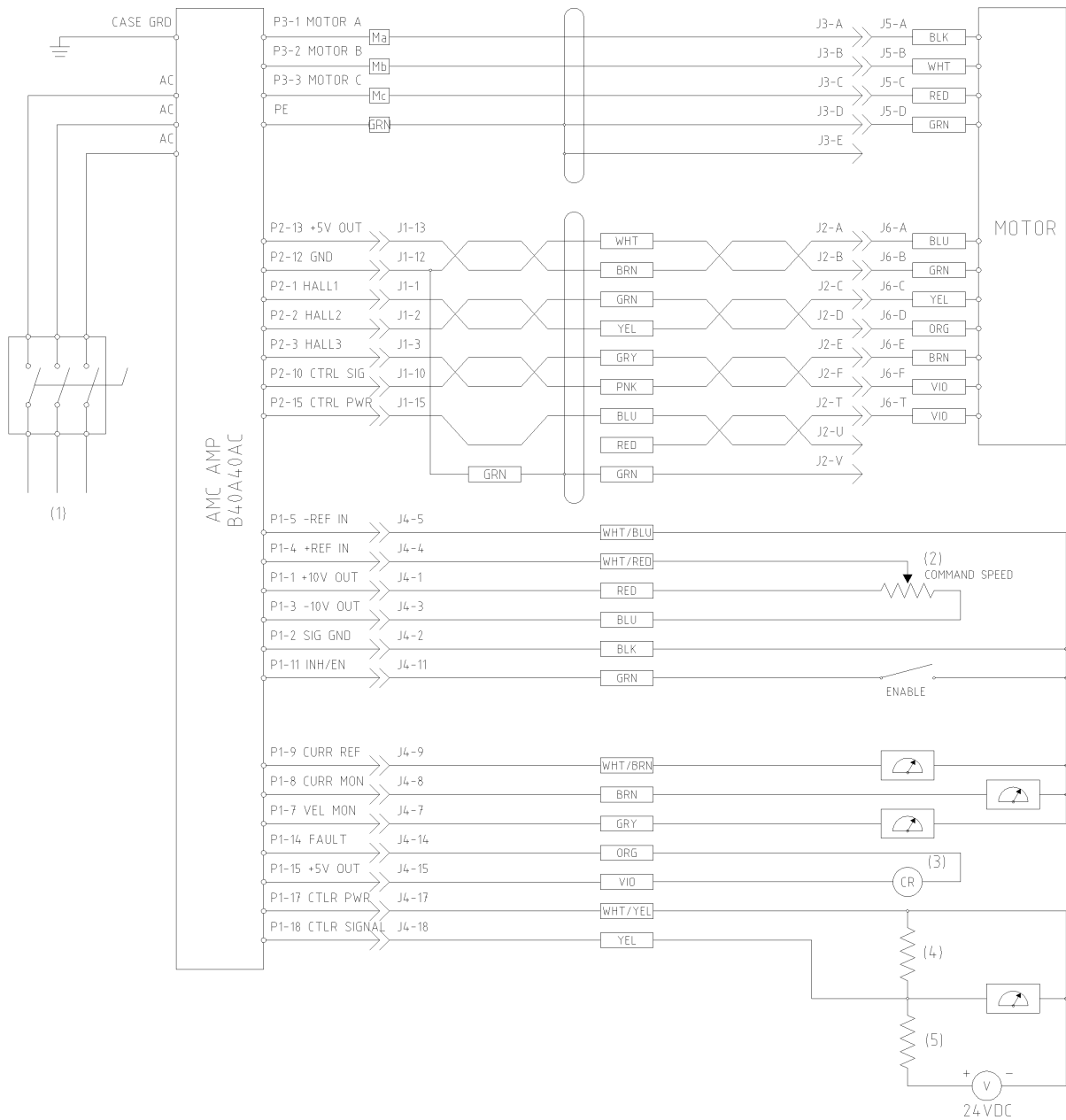
Figure 2. System Wiring Diagram
