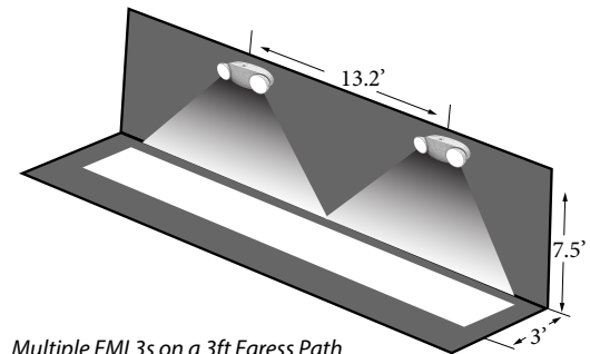
Multiple EML3s on a 3ft Egress Path
