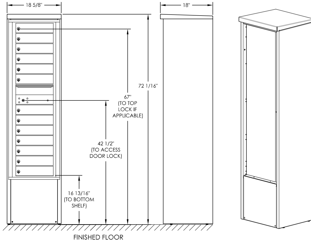
COMPARTMENT CHART
