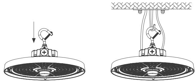
Hook Mount
